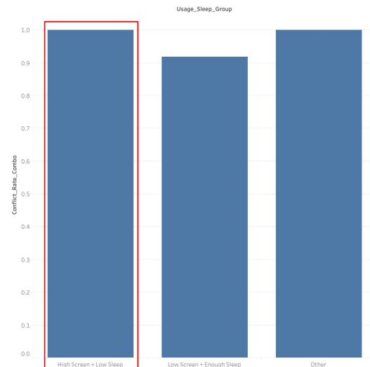
Screen Time & Sleep vs Conflicts
