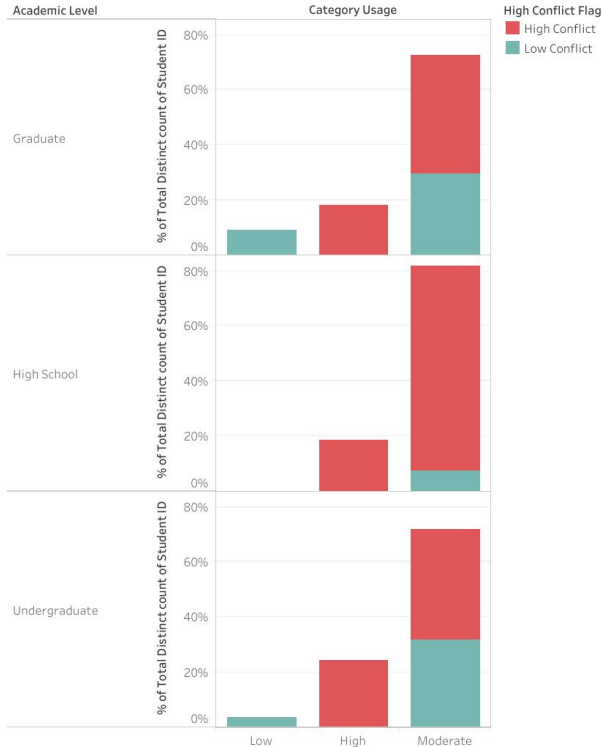
Stacked Bar: High Conflict Flag by Usage Category (2)
